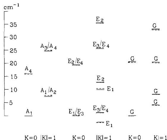
Figure 13. Comparison of computed and observed levels of NH 3 -NH 3 : dashed lines, computed; solid lines, observed. 11 The K = 0 ground level of each species A , E , and G is adjusted. In several cases the difference between computed and observed values is within the width of the lines.
