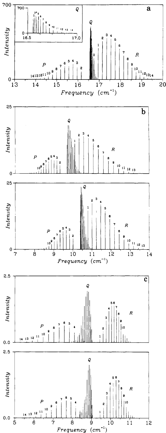
Figure 8. Rovibrational spectra calculated for (A) the lowest \Sigma \rightarrow \Pi transition in o -Ar-NH 3 and (B) the lowest \Sigma \rightarrow \Pi and (C) \Pi \rightarrow \Pi transitions in p -Ar-NH 3 from ref 8. Intensities in 10^{10} \text{ m}^2 \text{ s}^{-1} \text{ mol}^{-1} ; temperature 5 K. The two windows in the last two figures contain the spectra for the allowed E' \leftrightarrow E'' transitions between inversion doublets.
