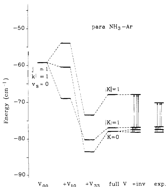
Figure 7. Calculated and experimental VRT levels of p - \text{Ar-NH}_3 . See the caption of Figure 6 for the explanation. The inversion splitting of the |K|=1 levels is so small that it is not visible here.
